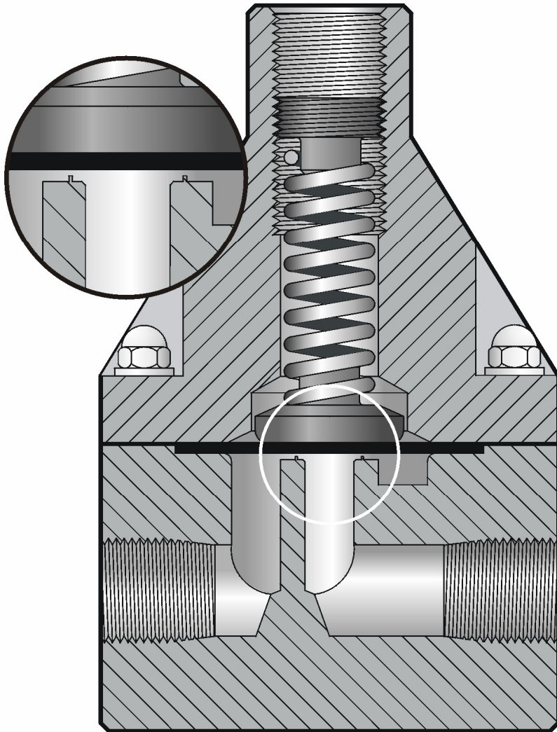
Back Pressure Valve
