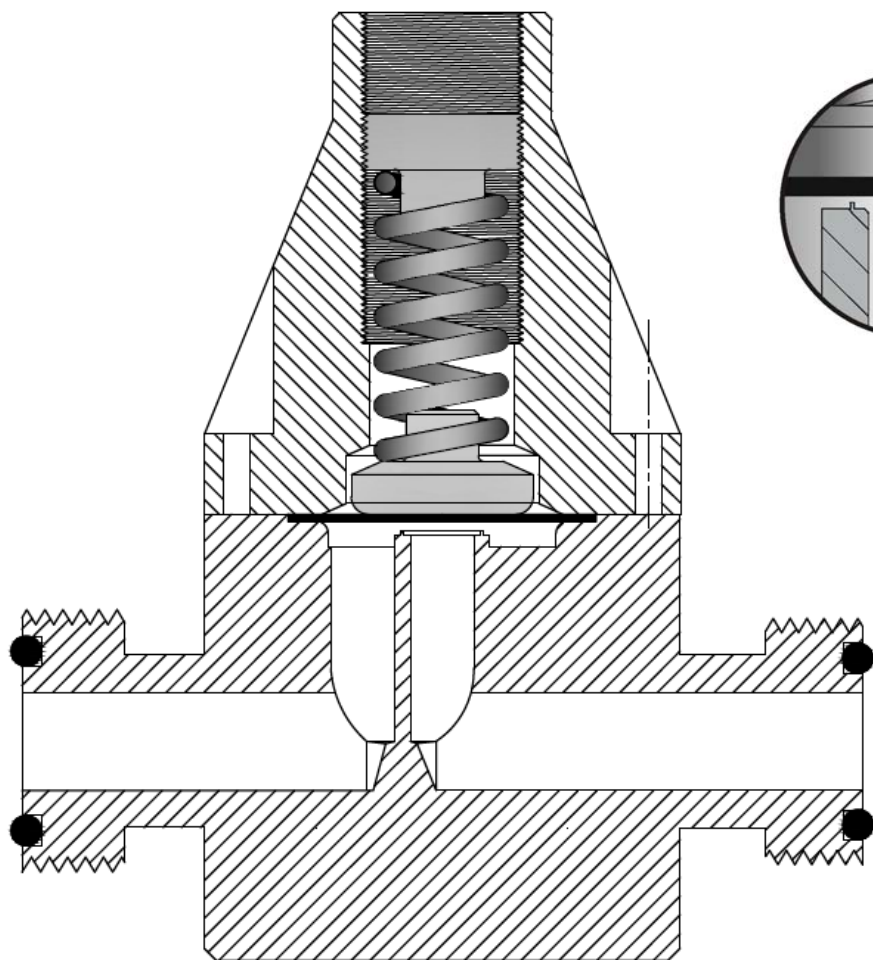
Back Pressure Valve
