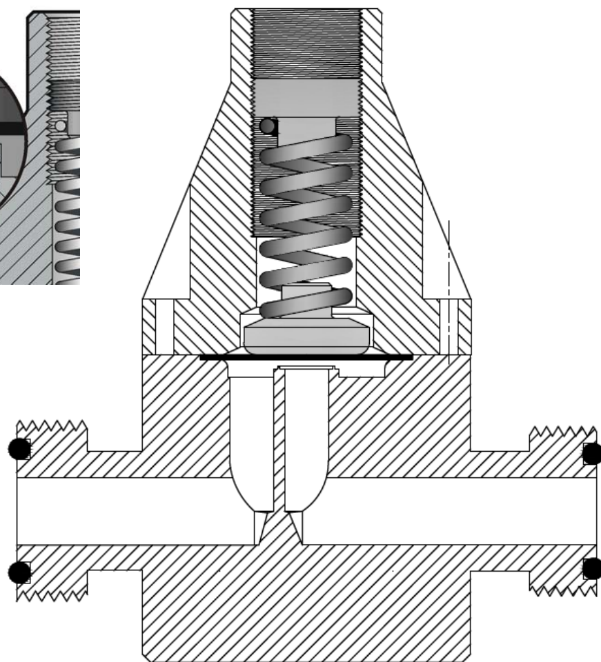
2 Port Pressure Relief Valve
