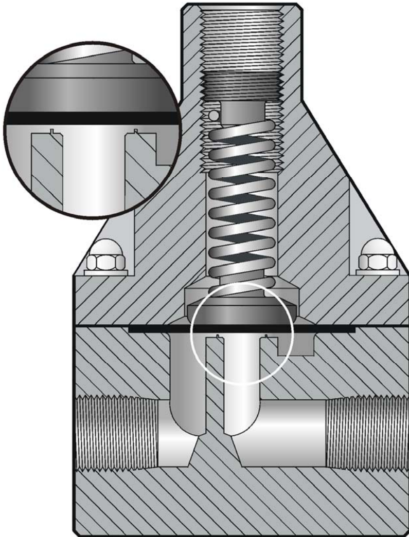
2 Port Pressure Relief Valve Flow is Left to Right
