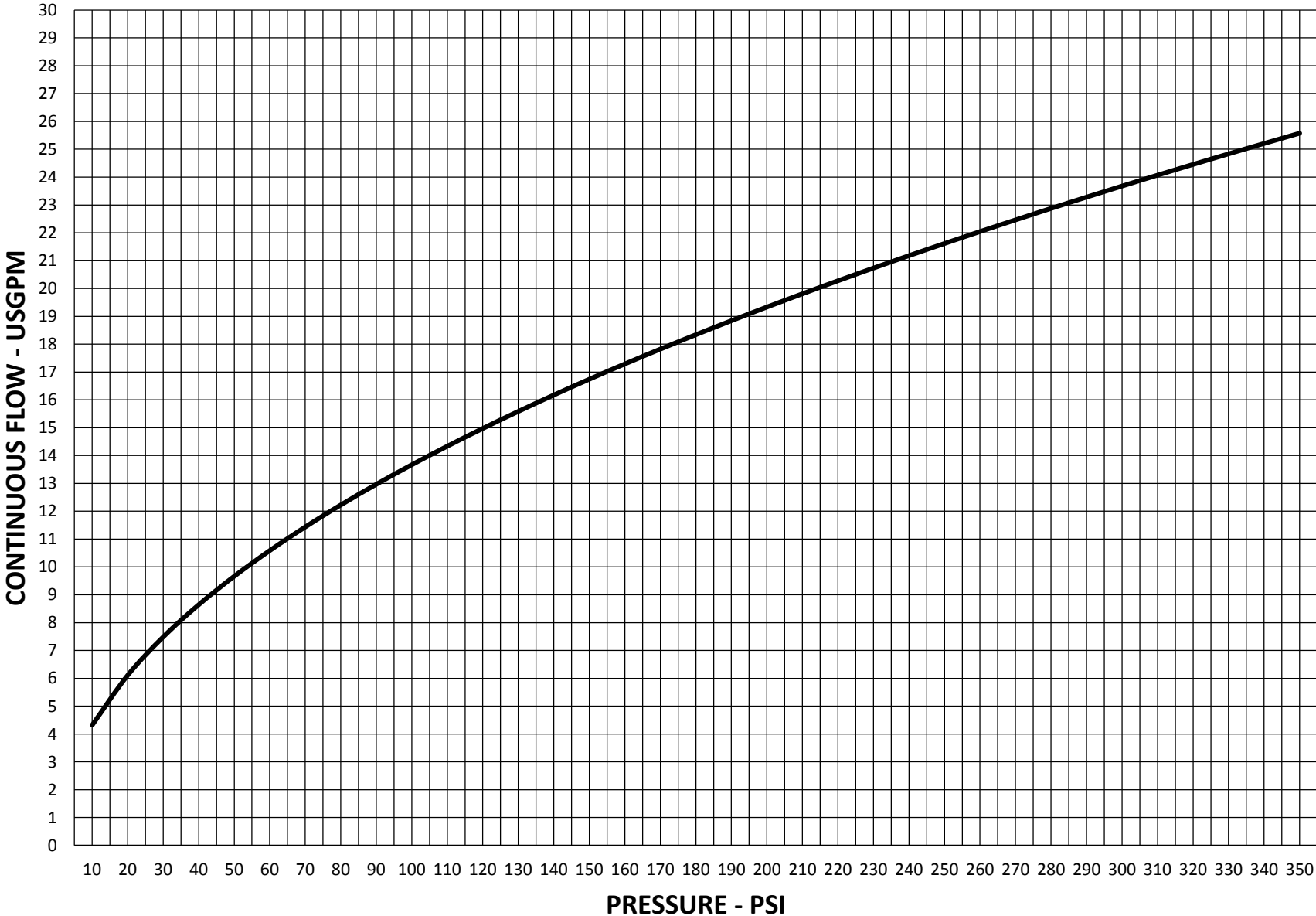
1/2" BPG / PRG - 350 psi Performance Curve
