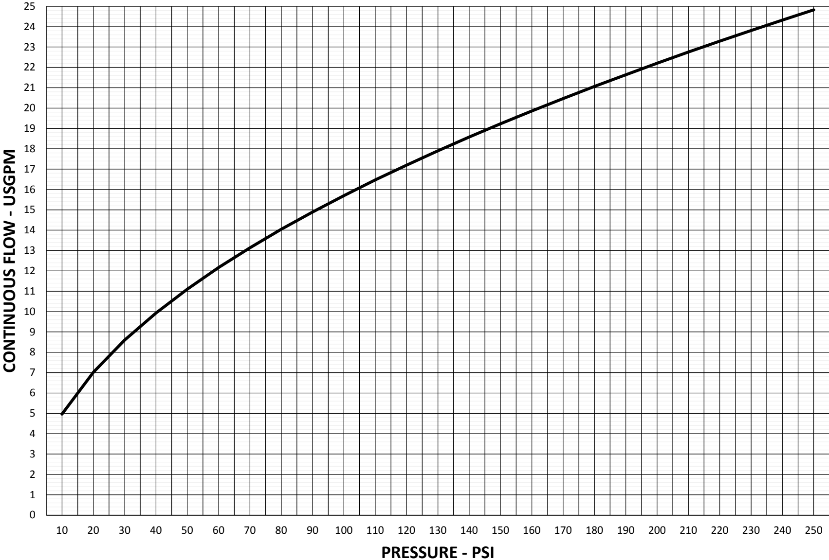
BPG / PRG 075 - 250 psi Performance Curve
