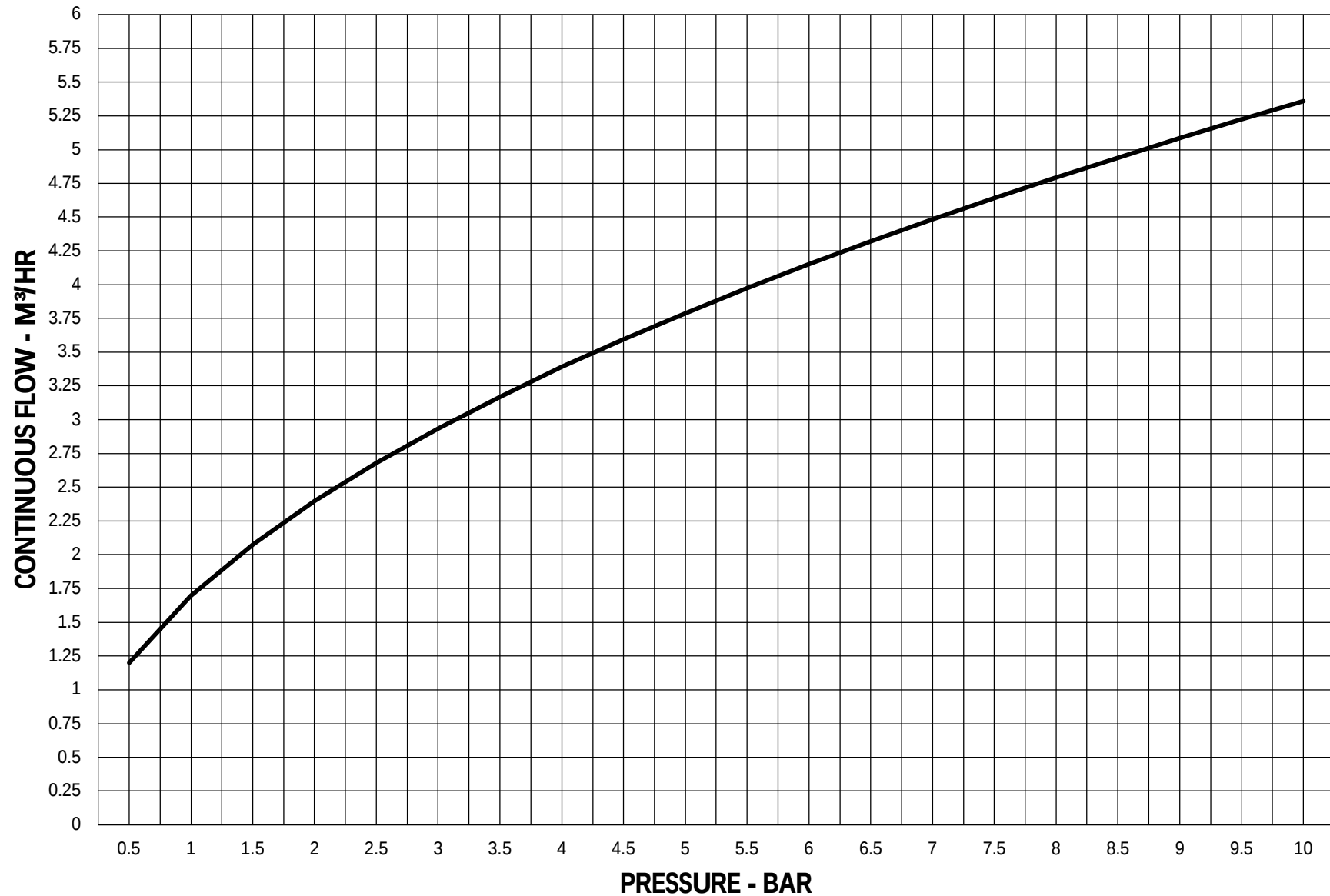
BPU / PRU 100 Performance Curve
