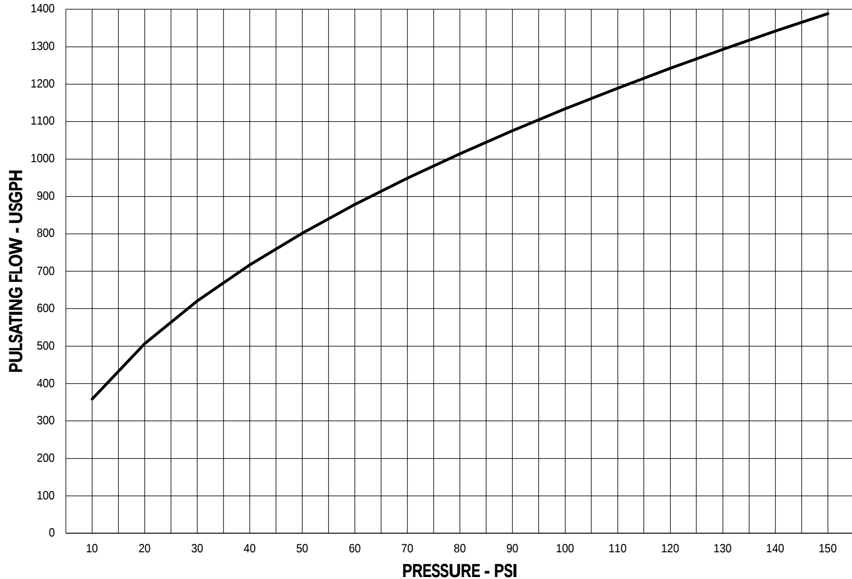
BPG / PRG 155 Performance Curve
