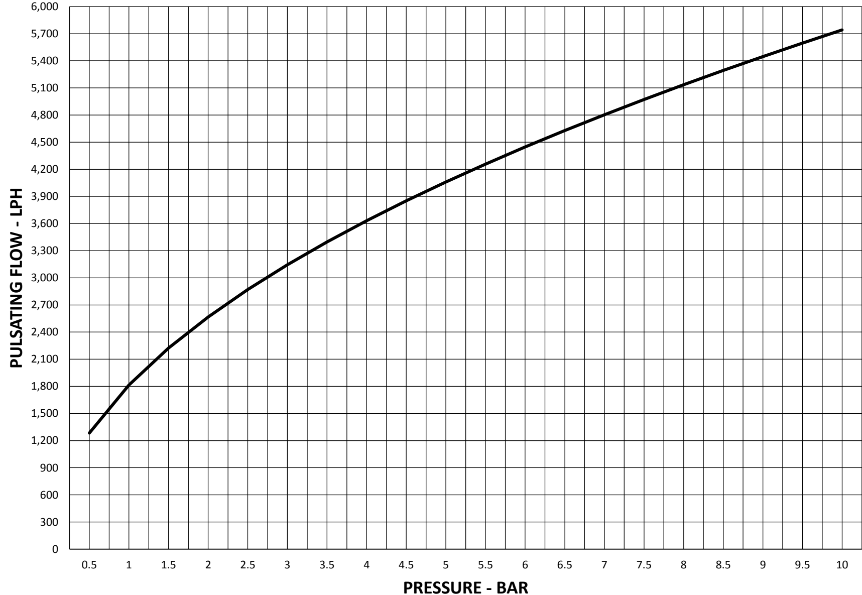
BPG / PRG 200 Performance Curve
