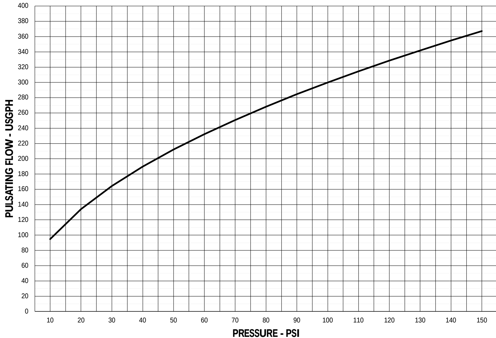
BPU / PRU 075 Performance Curve
