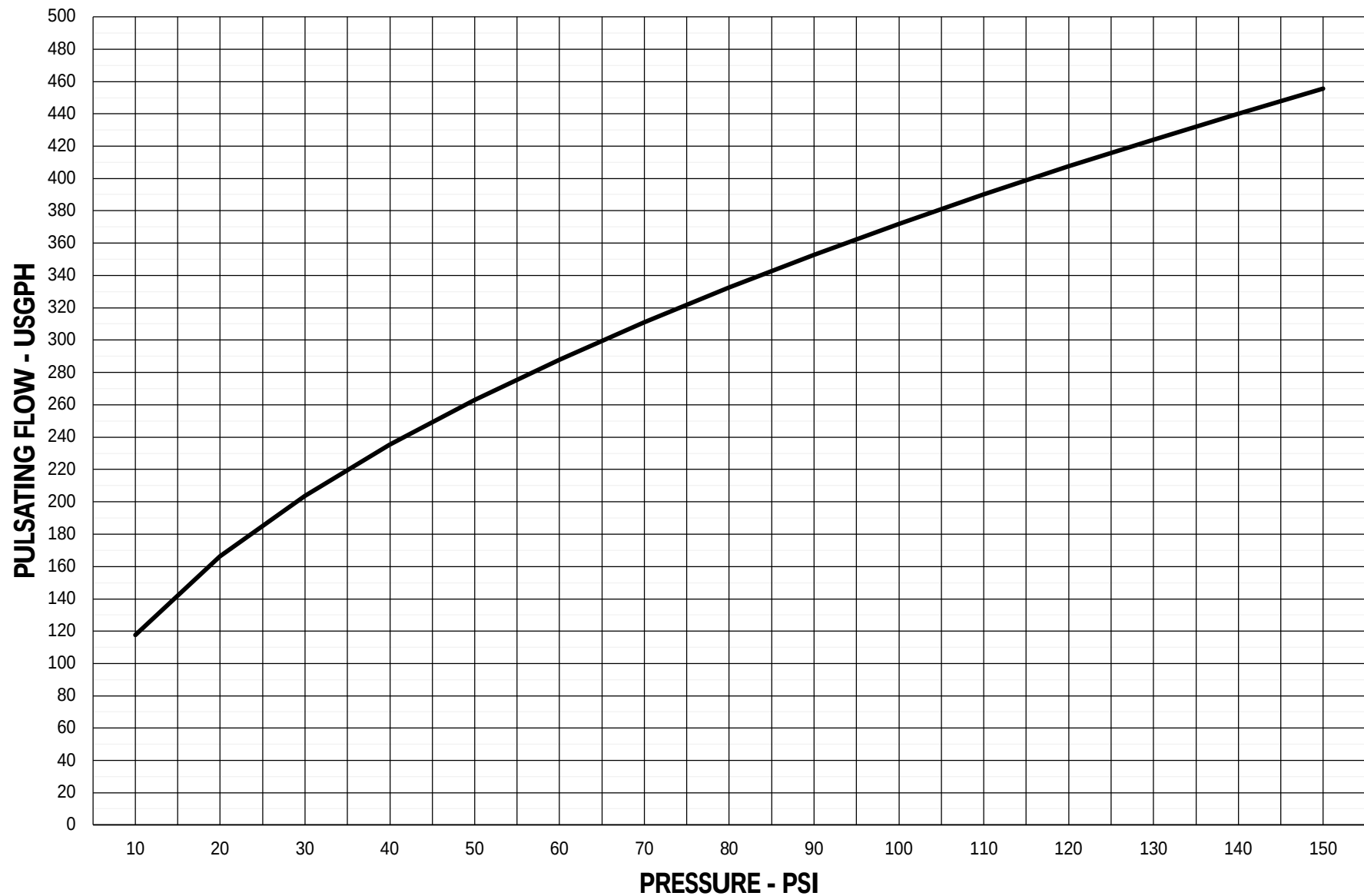
BPU / PRU 100 Performance Curve
